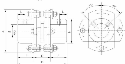
AZ-02,03,04 Type
