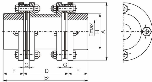
AX,A4-TYPE
