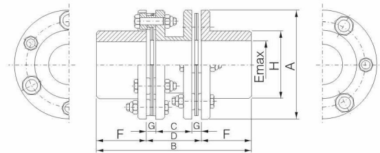
G4-TYPE
