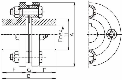
A3-TYPE
