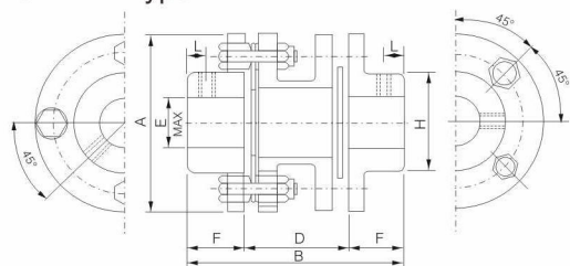
AB-04-NN Type
