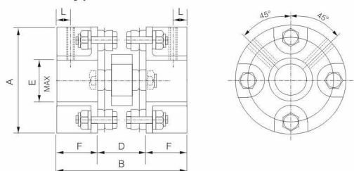
AZ-02-U Type
