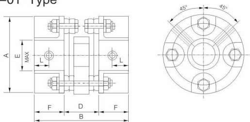
AZ-01 Type
